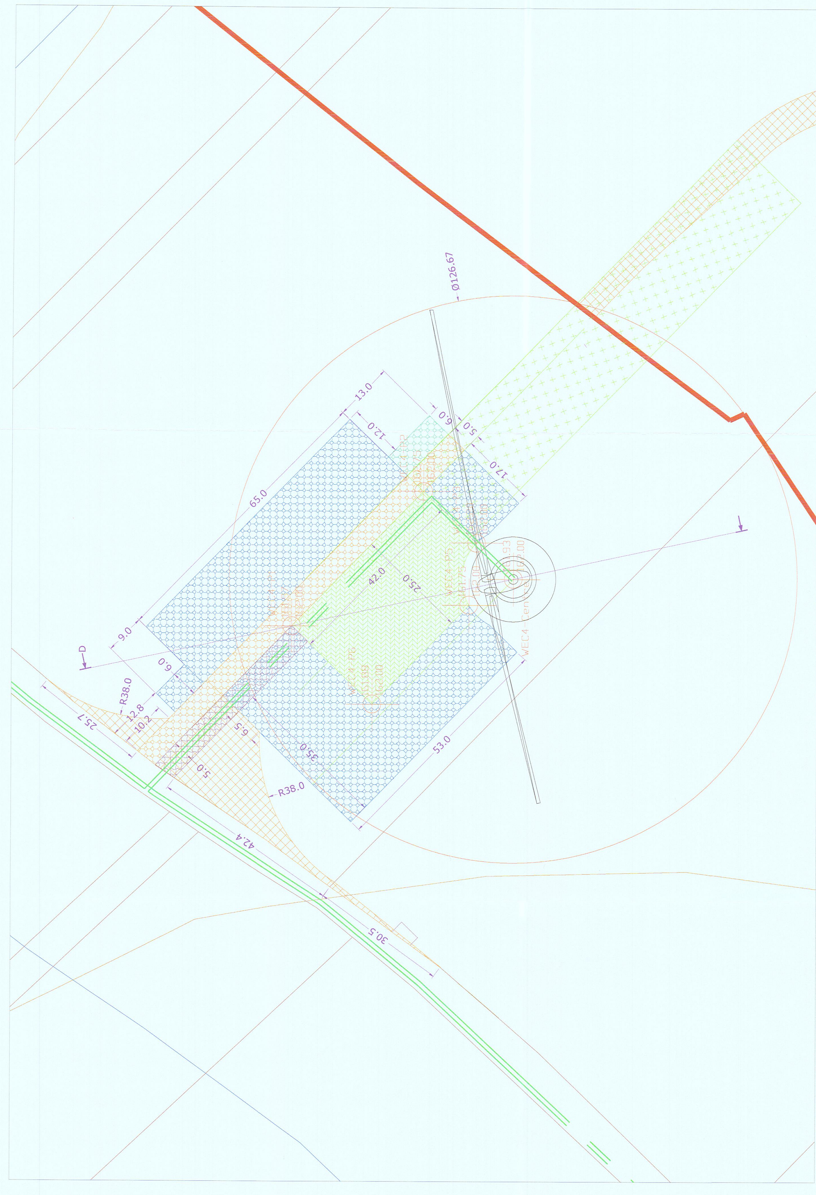
DETAIL EOLIENNE 4 (1/500)
